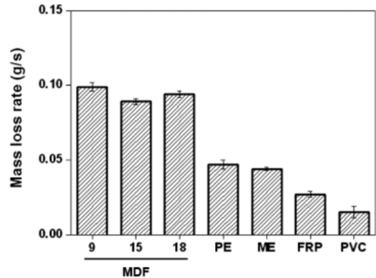
Fig. 5. Mass loss rate of testing flooring materials.
