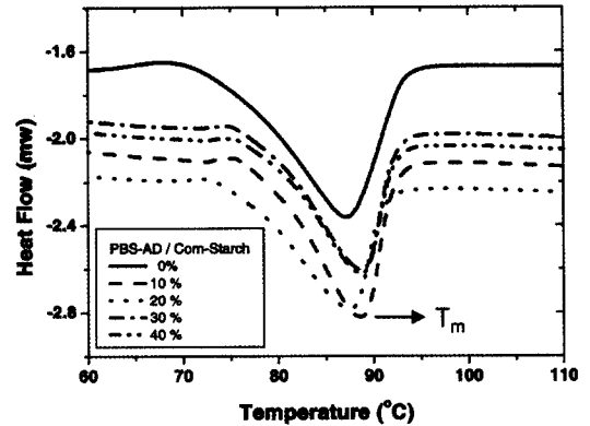
Fig. 6. DSC heating thermograms of corn-starch filled PBS-AD bio-composites.
